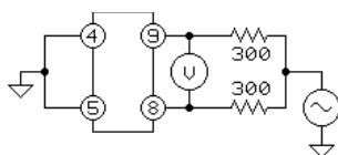
TEST CIRCUIT 2
