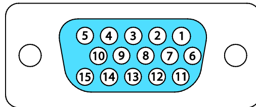
VGA PORT ON FLX-RI4
